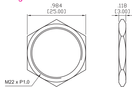
M22 bushing
