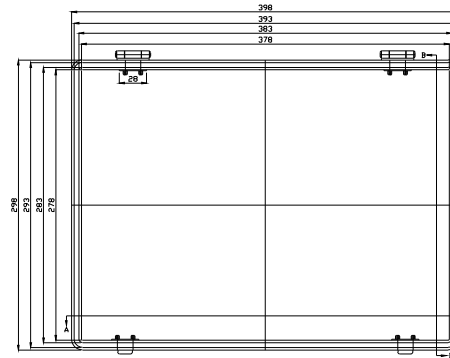
COVER-BOTTOM
