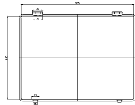
COVER-TOP
