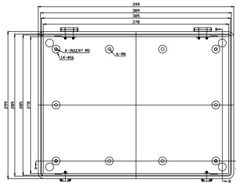
BODY-TOP
