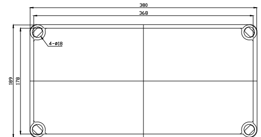
COVER-TOP
