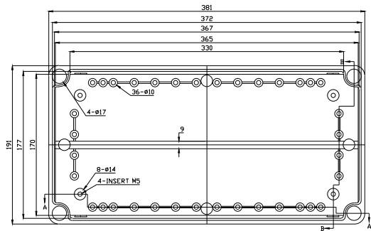
BODY-TOP
