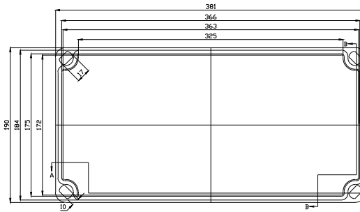
COVER-BOTTOM
