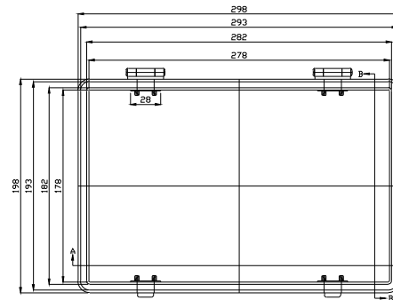
COVER-BOTTOM
