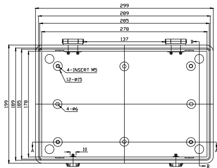
BODY-TOP
