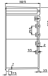
SECTION B-B
