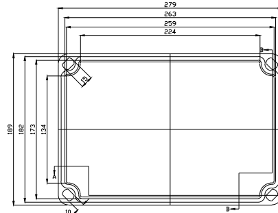
COVER-BOTTOM
