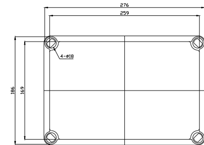
COVER-TOP
