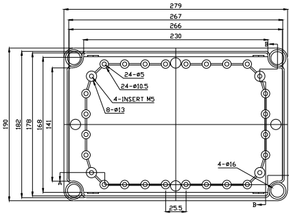
BODY-TOP
