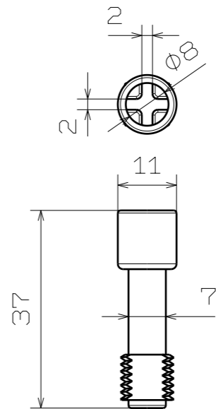
COVER BOLT
