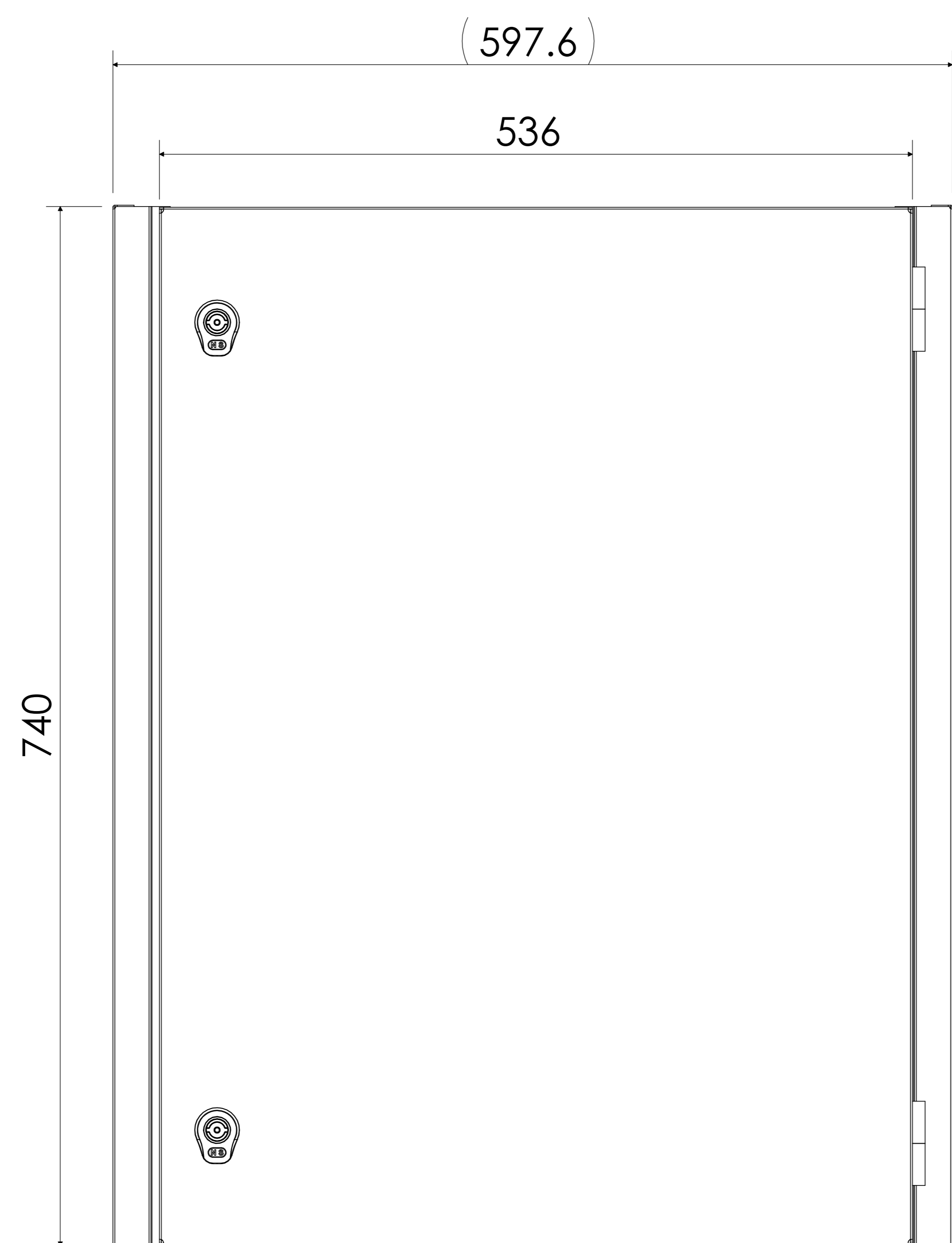
FRONT VIEW
