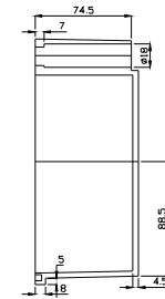
SECTION B-B
