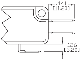
C TYPE (QUICK CONNECT .187 series)
