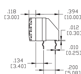
P.C.MOUNTING
