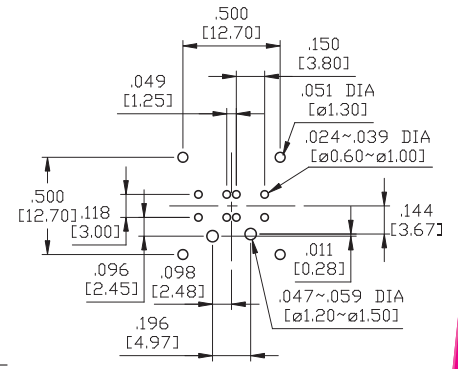
P.C.B Mounting
