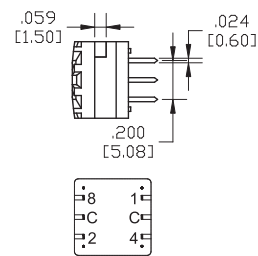
P.C.MOUNTING
