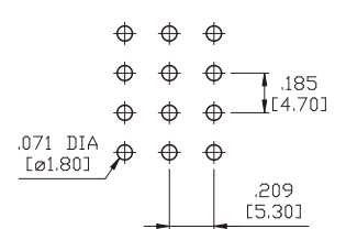
4P
