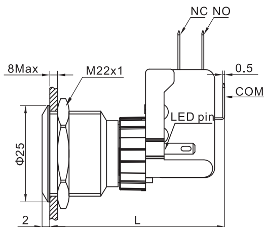
Illuminated Ring
