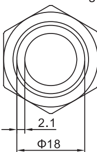
Illuminated Ring
