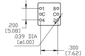
P.C.MOUNTING
