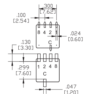
SURFACE MOUNTING
