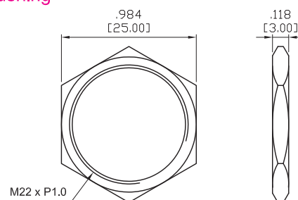
M22 bushing
