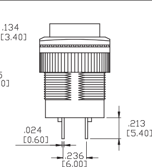
P.C.MOUNTING
