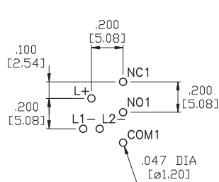
2 LEDs
