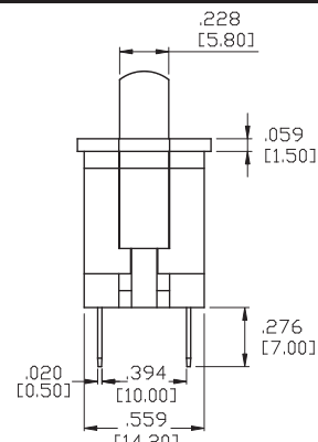
P.C.MOUNTING
