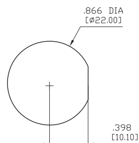
M22 x 1.0 FLAT-CUT THD. BUSHING
