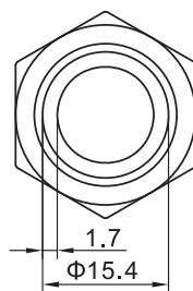
Illuminated Ring
