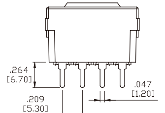
4P
