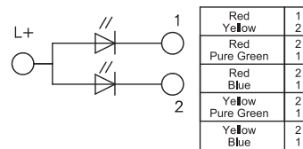
Dual colors LED
