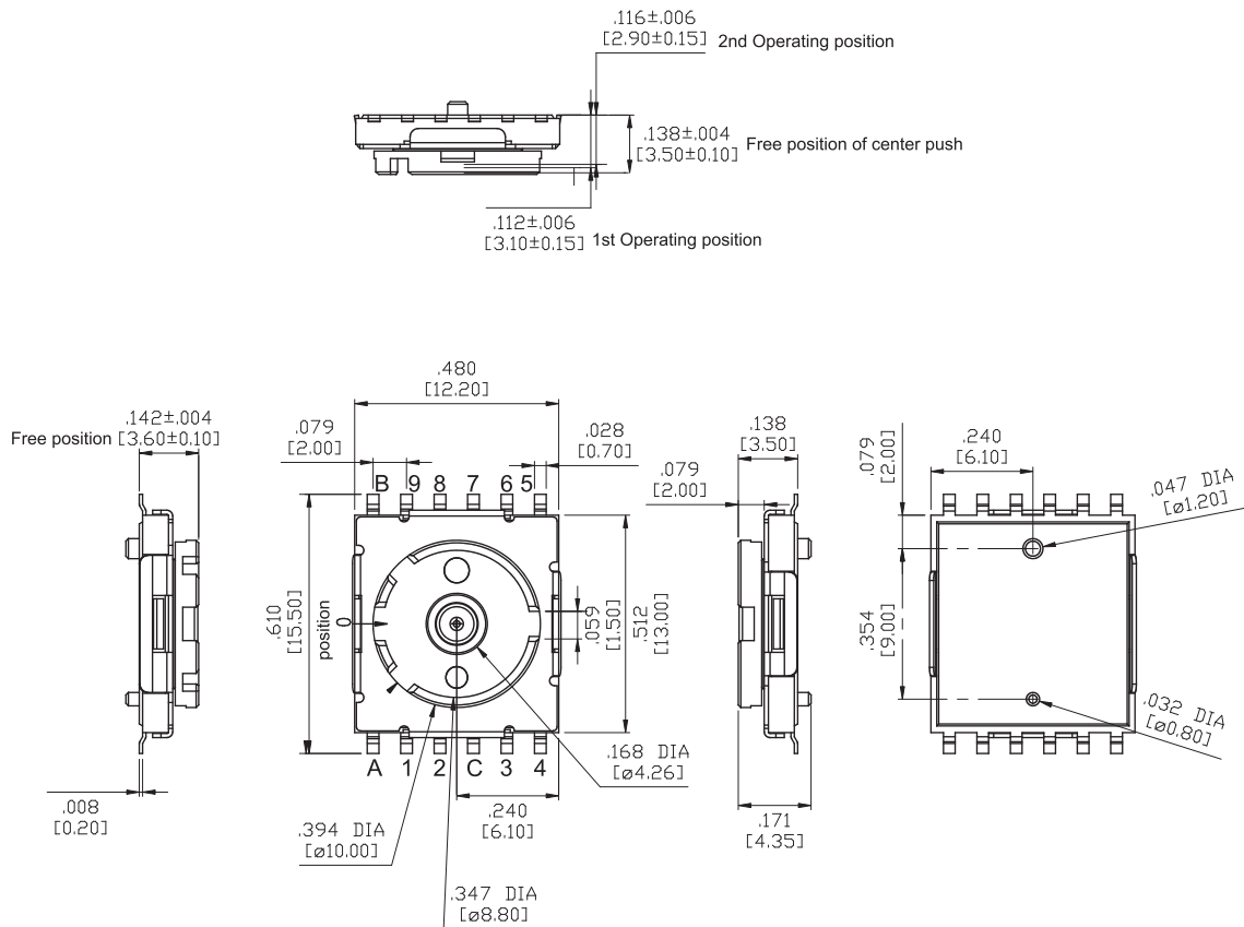
P.C.B MOUNTING
