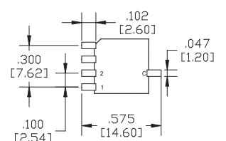
SURFACE MOUNTING
