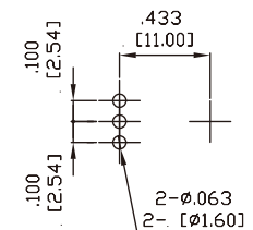
Dual Colors PCB Mounting Layout
