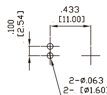
Single Color PCB Mounting Layout
