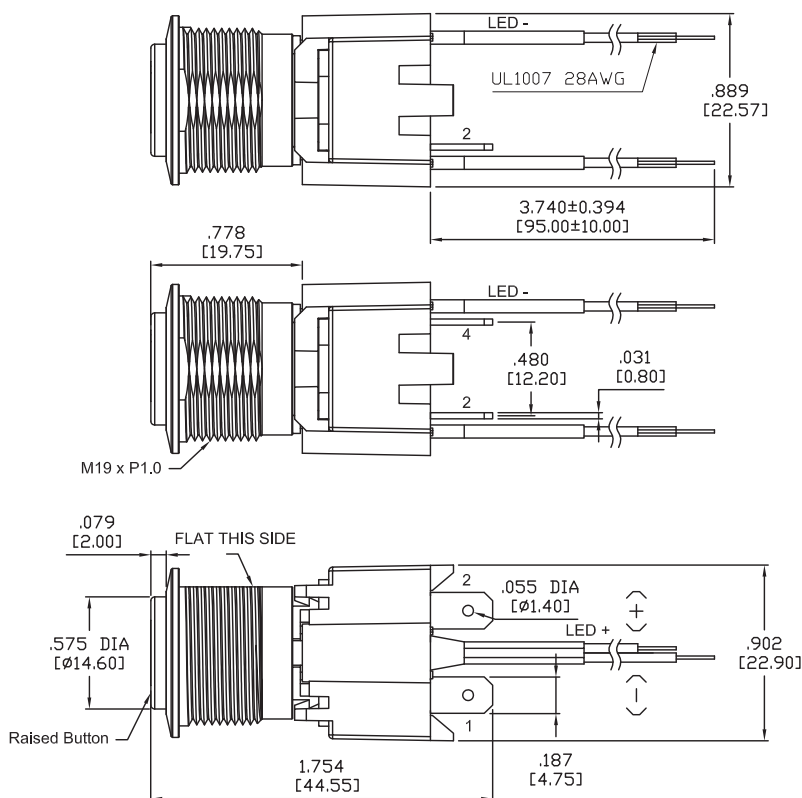
Schematic
