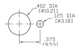
METRIC BUSHING
