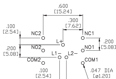
2 LEDs
