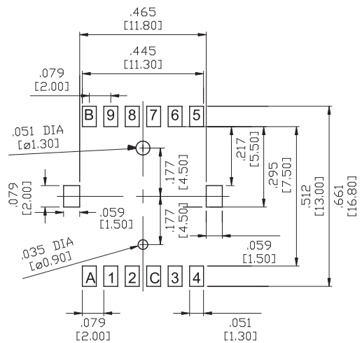
P.C.B MOUNTING
