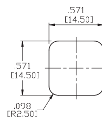
P.C.MOUNTING
