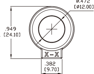
DIMENSIONS OF THE LED RING
