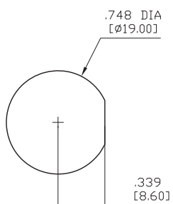
M19 x 1.0 FLAT-CUT THD. BUSHING
