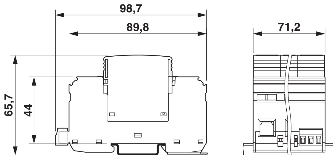
Dimensional drawing
