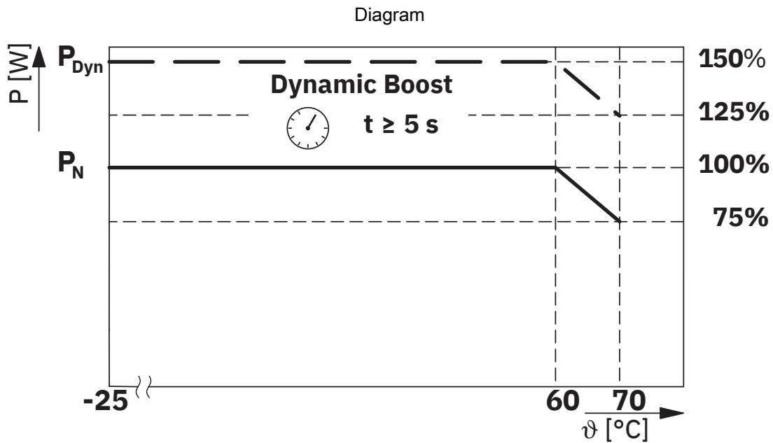
Temperature-dependent derating
