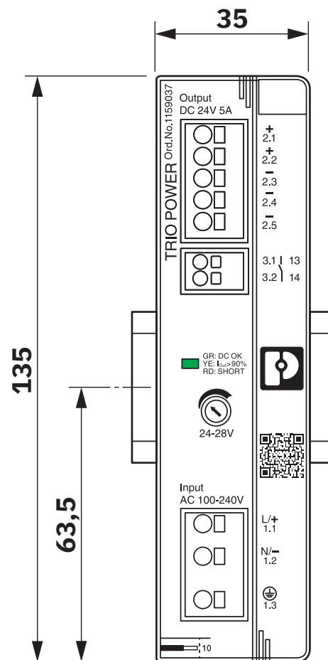
Dimensional drawing
