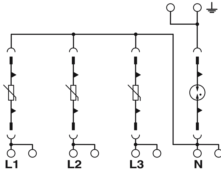
Circuit diagram
