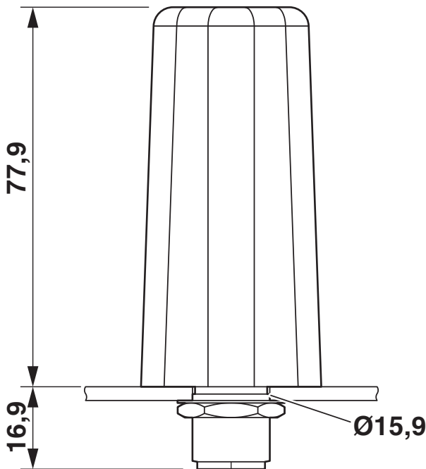
Dimensional drawing
