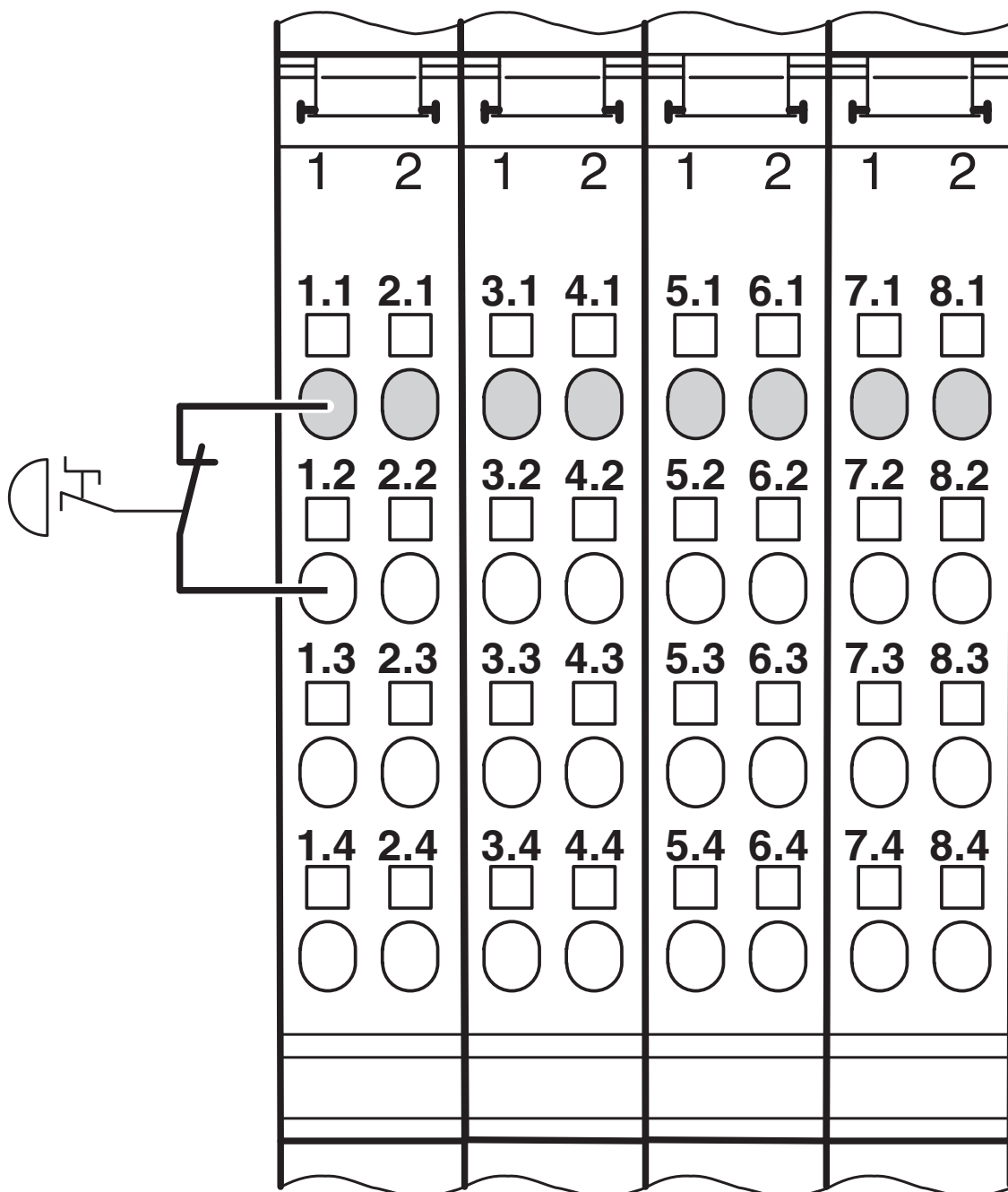
Connection example for an emergency stop circuit
