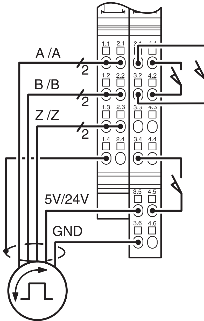
Connection diagram
