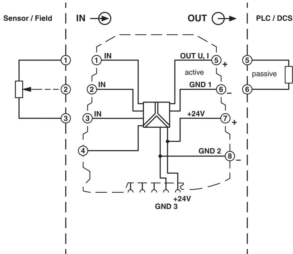
Block diagram
