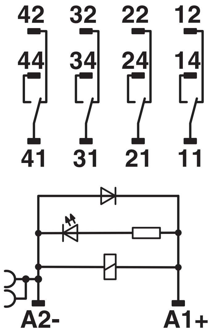
Circuit diagram
