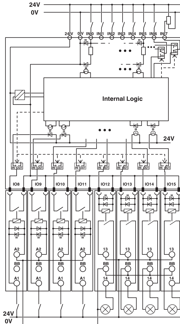
Circuit diagram
