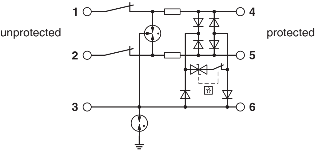
Circuit diagram
