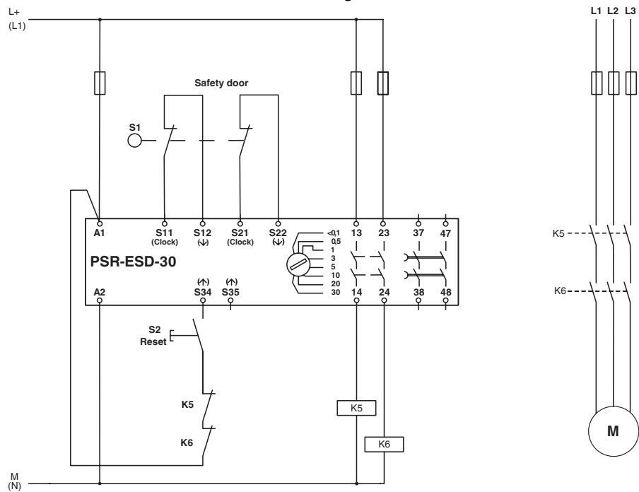
Circuit diagram
