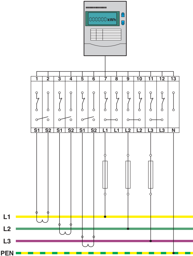
Circuit diagram
