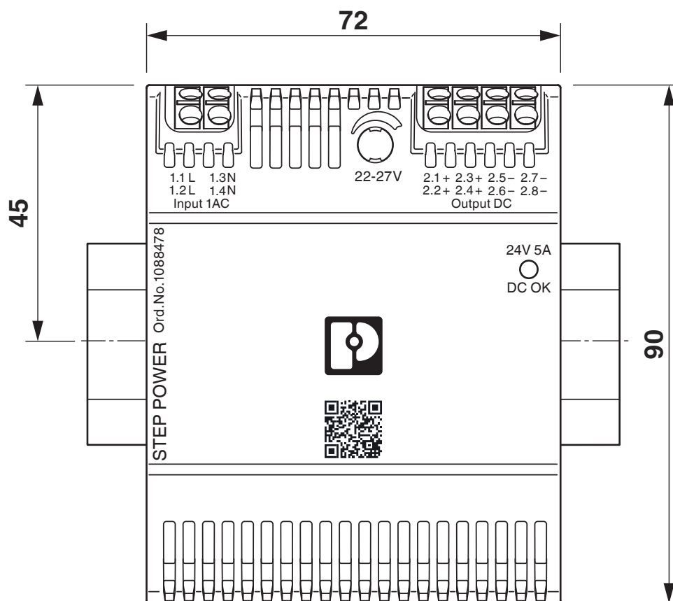
Dimensional drawing
