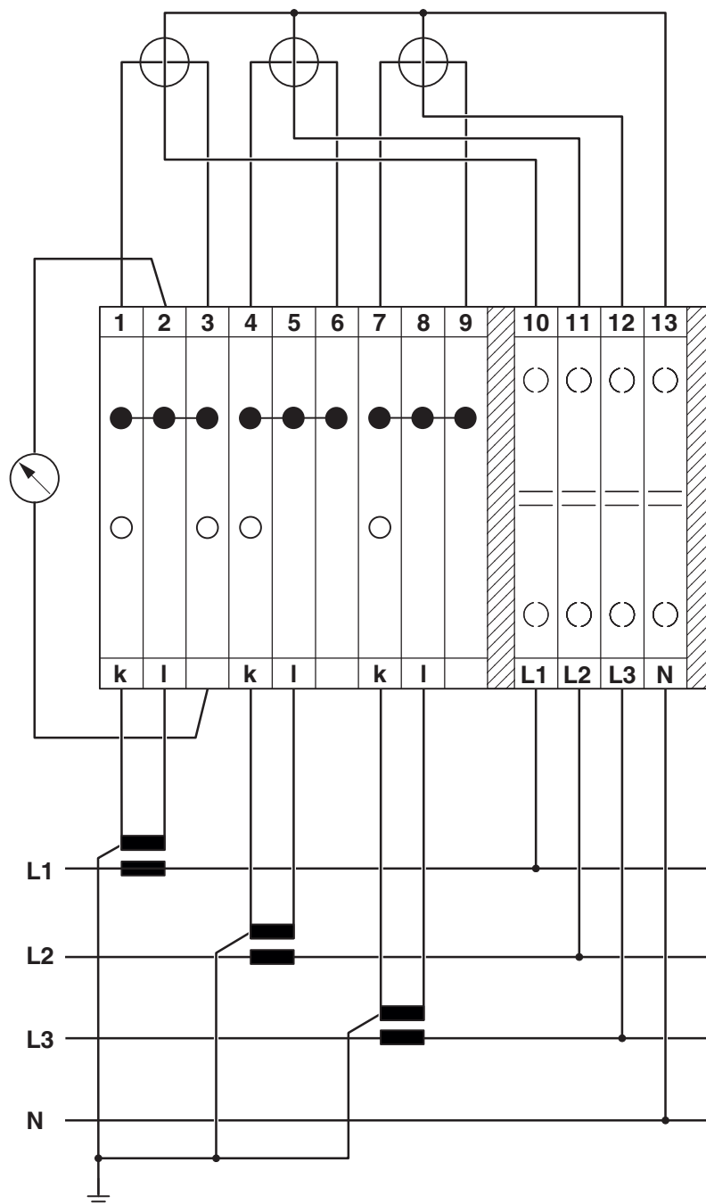
Schematic diagram
