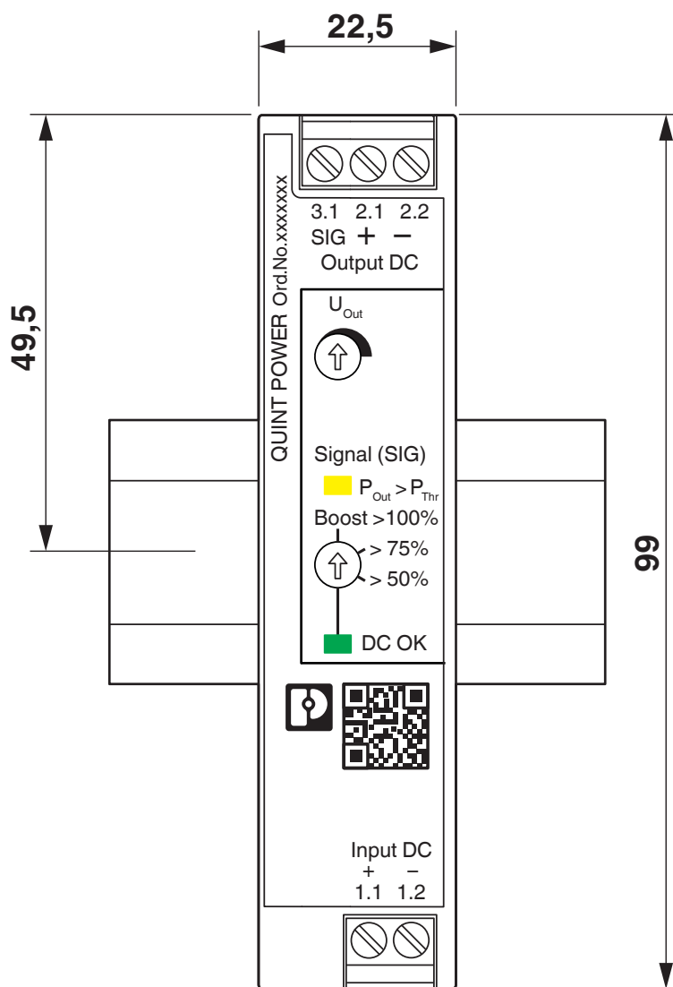
Dimensional drawing
