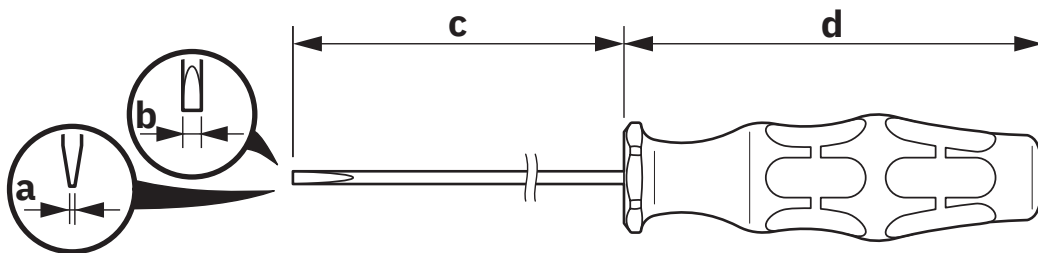
Dimensional drawing
