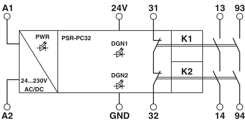
Block diagram
