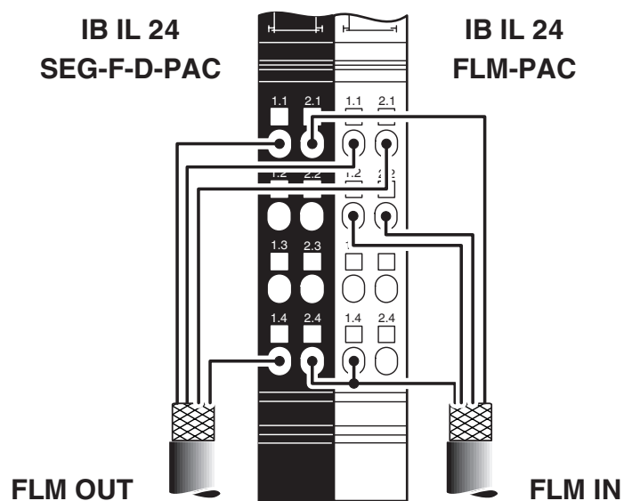
Connection diagram
