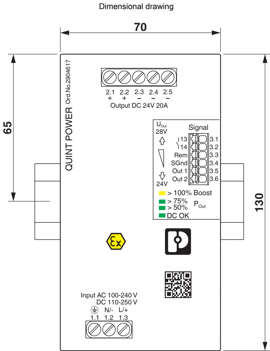
Device dimensions (dimensions in mm)
