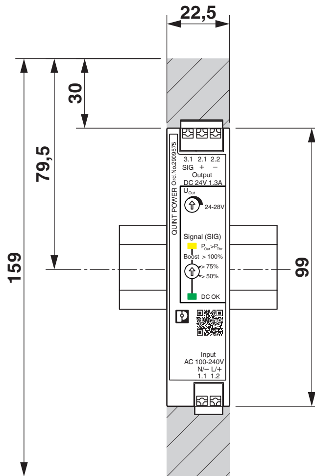
Dimensional drawing
