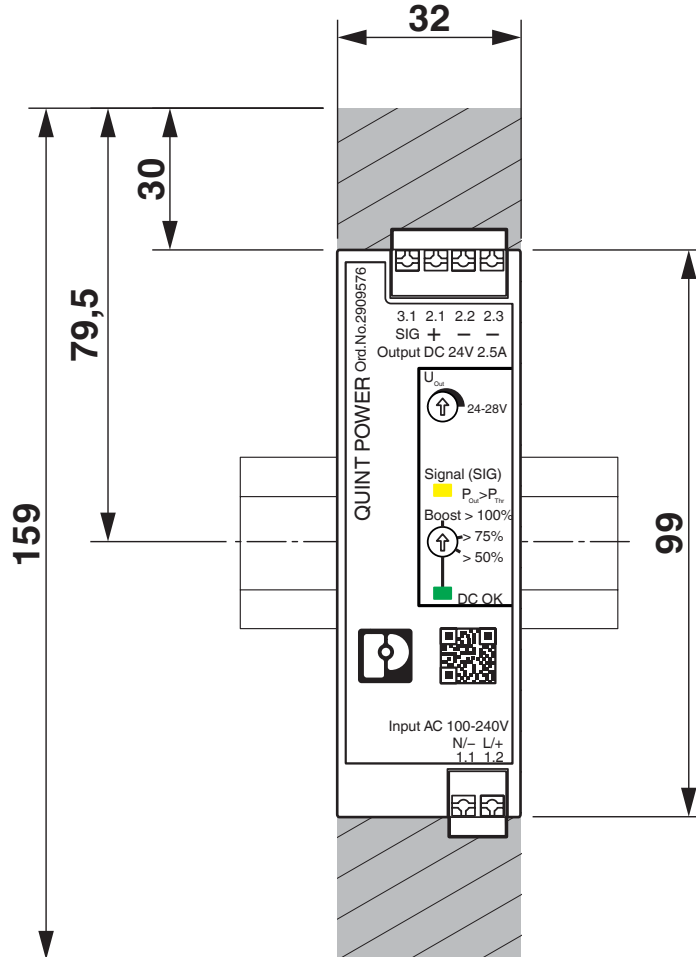
Dimensional drawing
