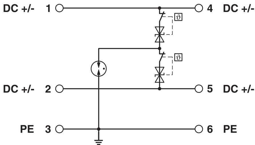
Circuit diagram
