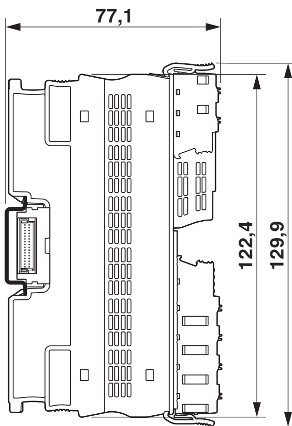
Dimensional drawing
