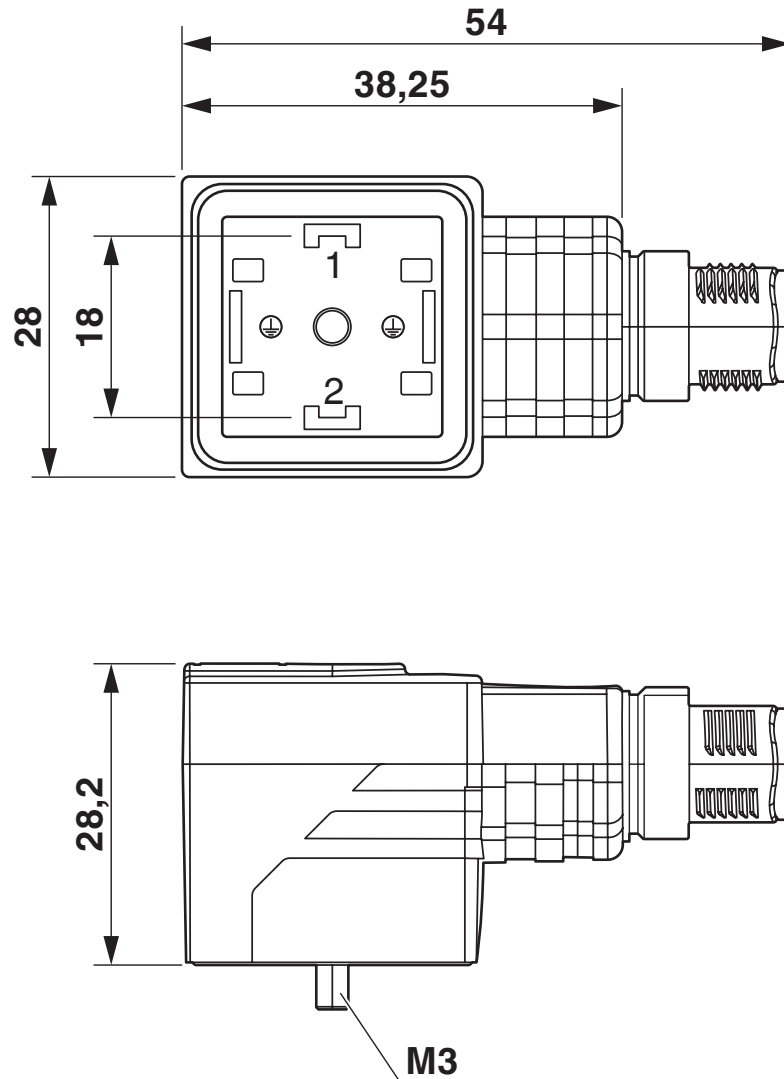
Dimensional drawing
