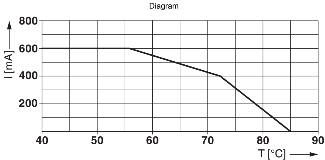
Diagram Derating for Ex-areas (Zone 2, EX ec)
