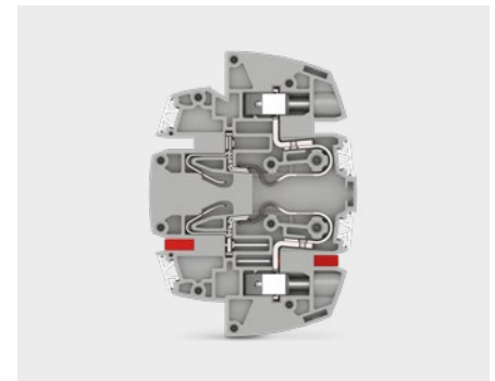
FAME 1 plug-in test socket
