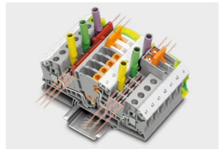
Transformer terminal block with six function shafts
