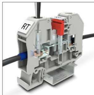
Terminal block with RT bolt connection
