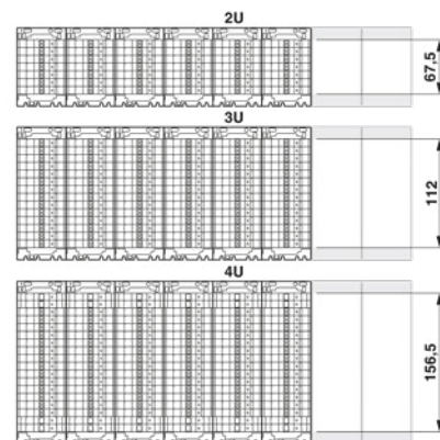
Rack units of the FAME 3 RACK
