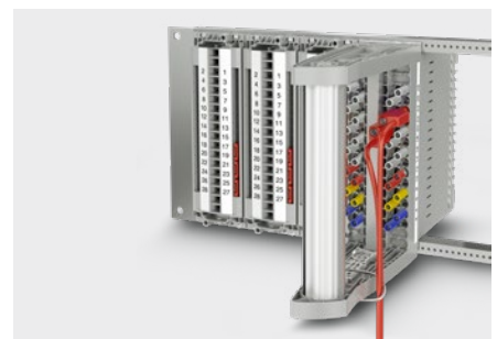
Test plug of the FAME 3 RACK system
