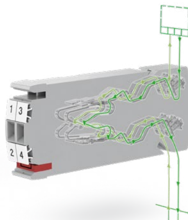
FAME RACK
