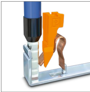
Clamping principle of a push-in terminal block
