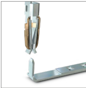
Clamping part of a plug-in COMBI terminal block
