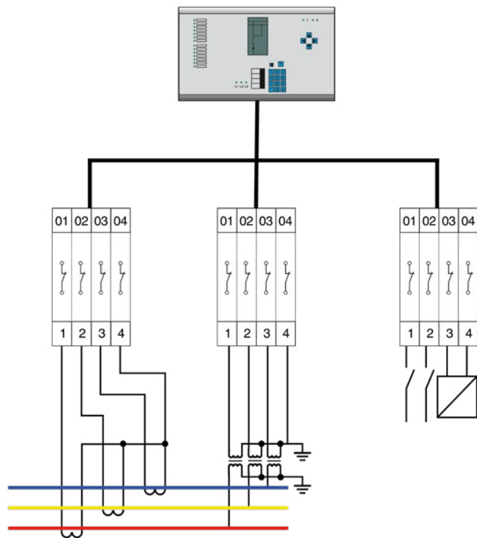
Plug-in test socket for voltage transformers
