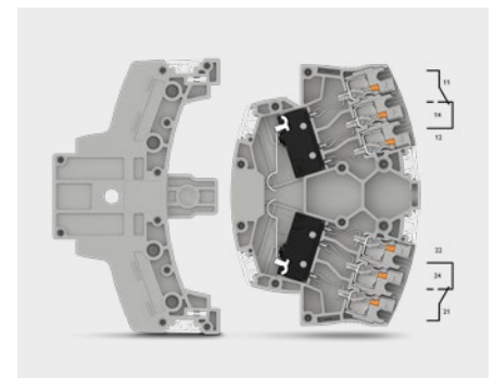
Plug-in test socket with status indicator
