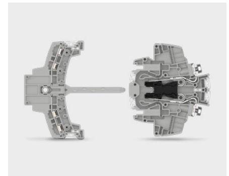
FAME 3 auxiliary contact for status recognition
