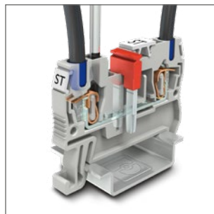
Terminal blocks with ST spring-cage connection
