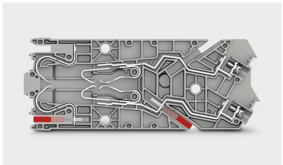
Single block of the FAME 3 RACK plug-in test socket
