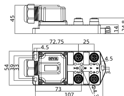
• Four-hole junction box without cable
