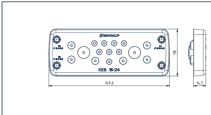
Dimensional diagram
