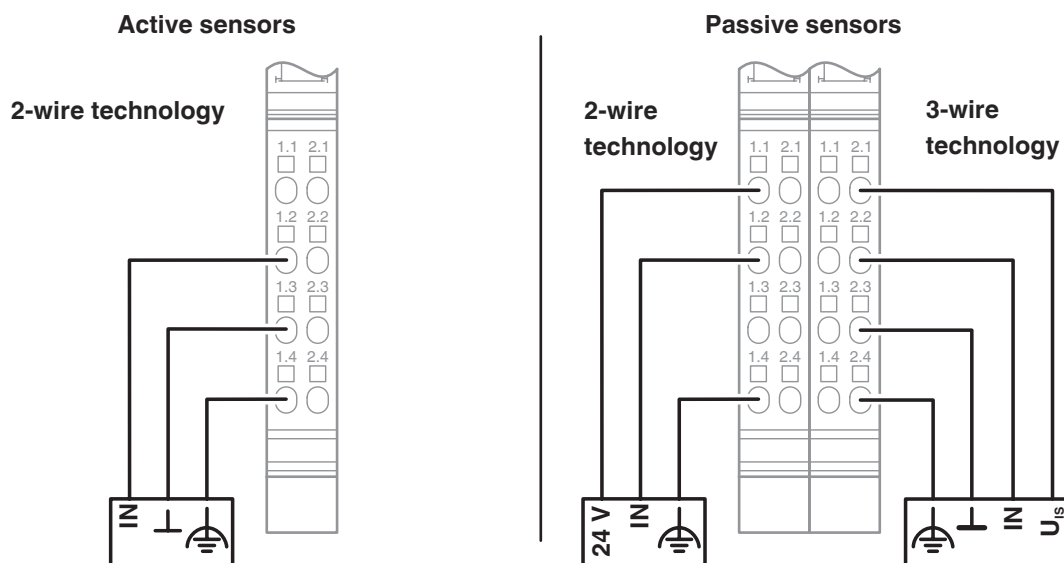
Connection diagram
