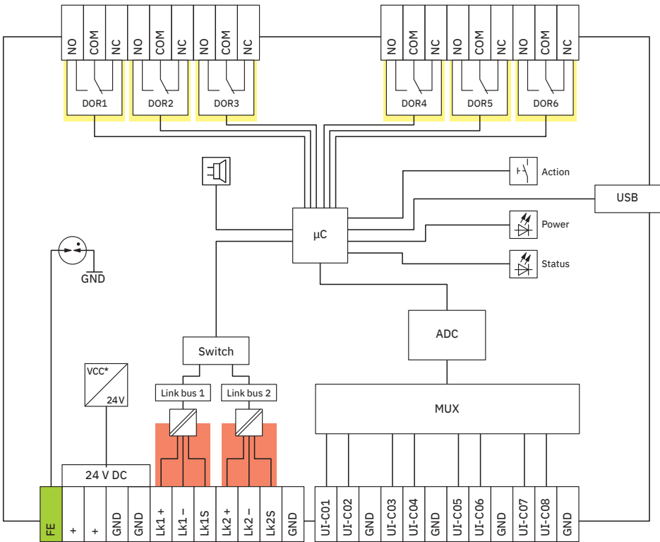
Block diagram
