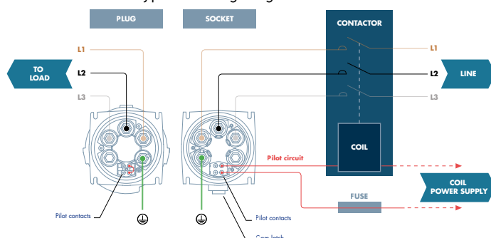
Typical wiring diagram of the DS4 control circuit
