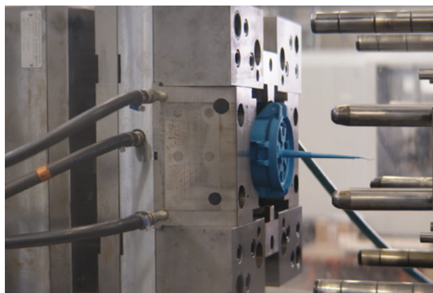
INJECTION PROCESS
