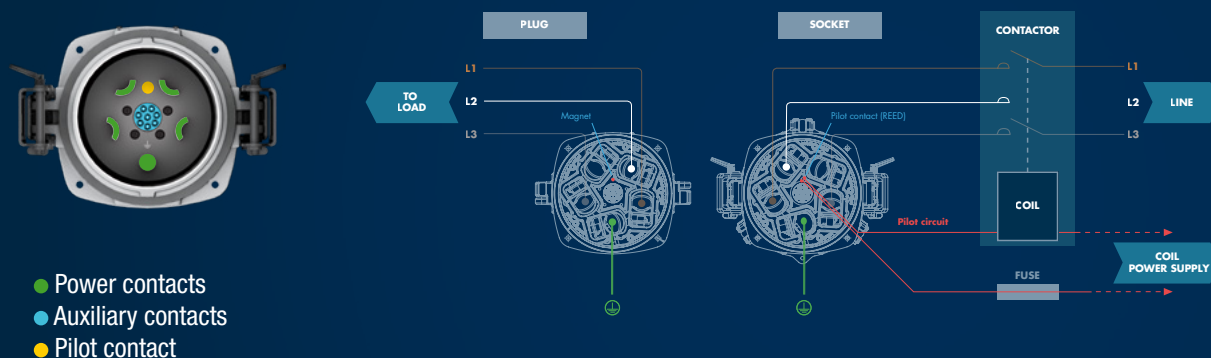
Typical wiring diagram of the P66 control circuit
