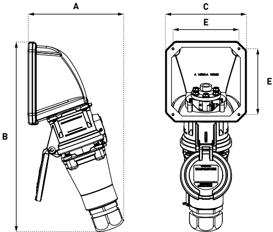
PLUG ON 70° INCLINED SOCKET-OUTLET
