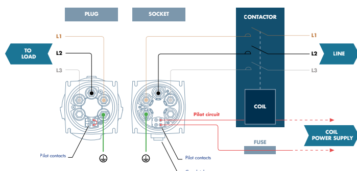
Typical wiring diagram of the DS2 control circuit
