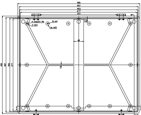
BODY-TOP
