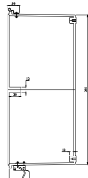
SECTION B-B
