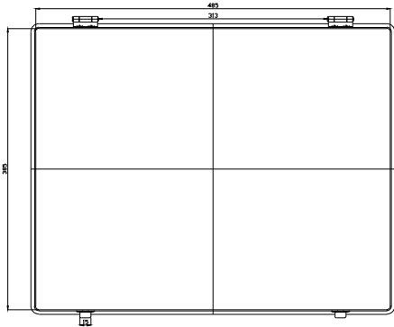
COVER-TOP
