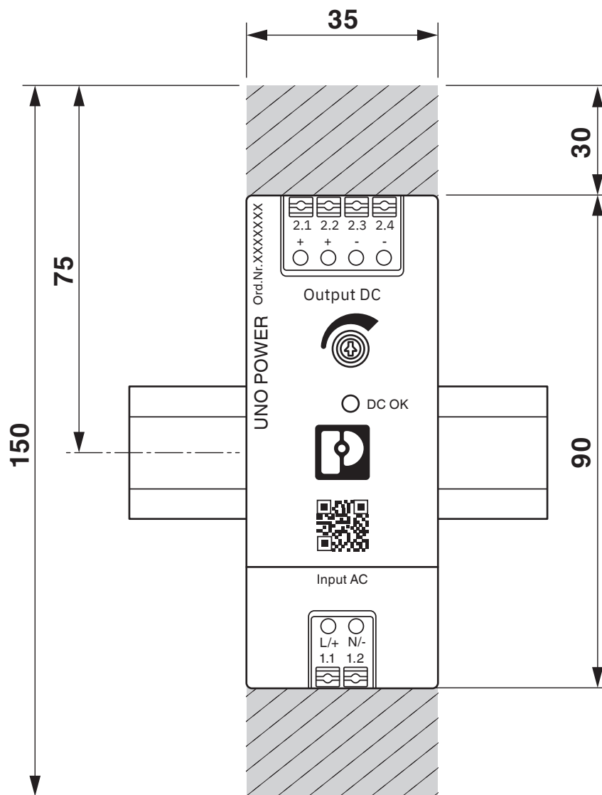
Dimensional drawing
